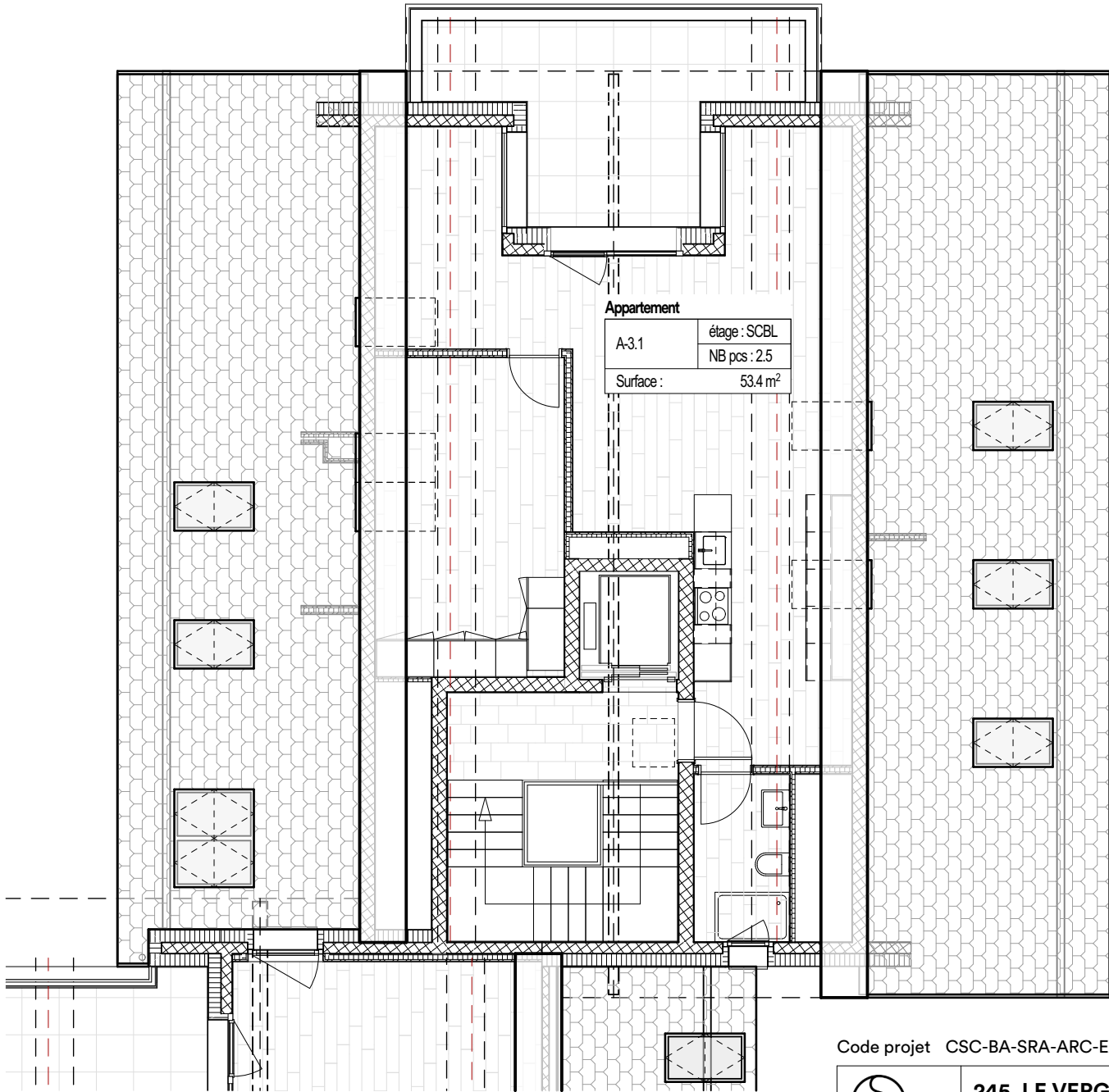
Surcombles
